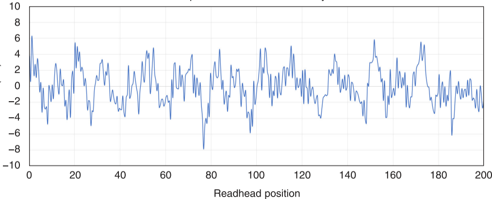
Interpolated error – 10 encoder cycles
