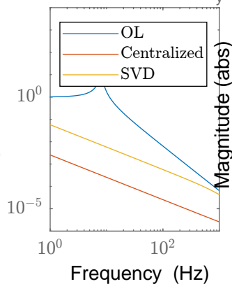
Bode Diagram
