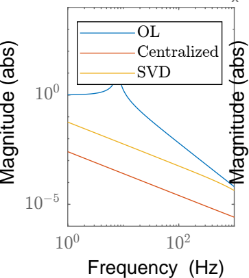
Bode Diagram
