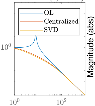
Bode Diagram
