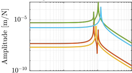
Diagonal elements of the Plant
