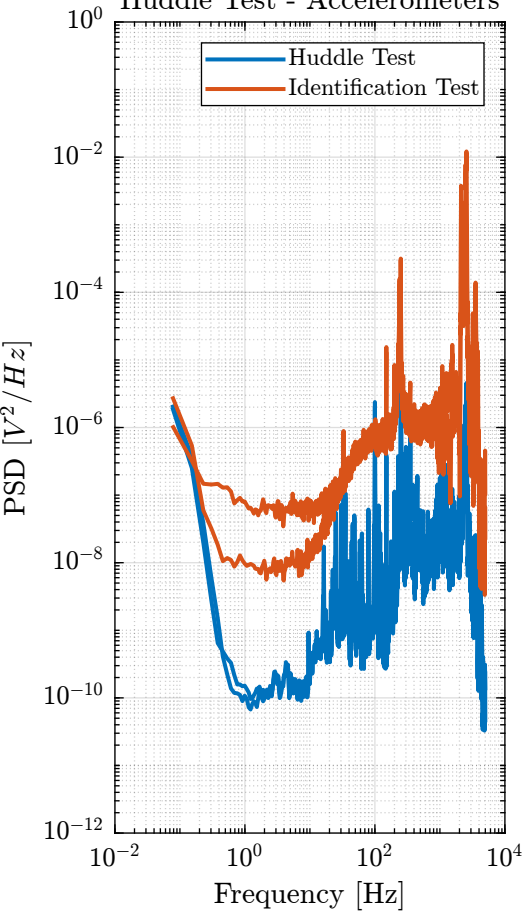
Huddle Test - Accelerometers
