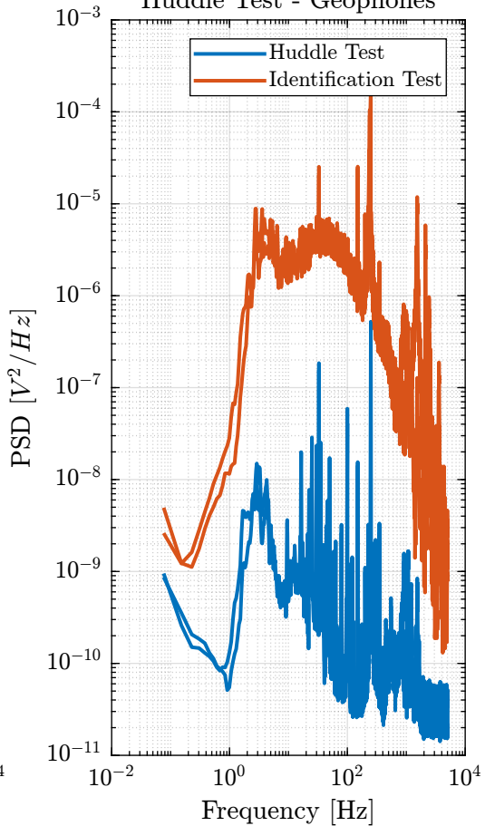
Huddle Test - Geophones
