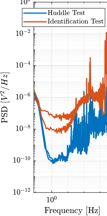
Huddle Test - Accelerometers
