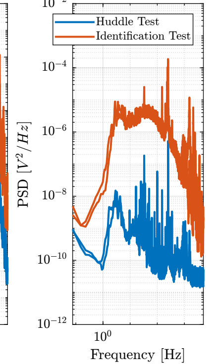
Huddle Test - Geophones
