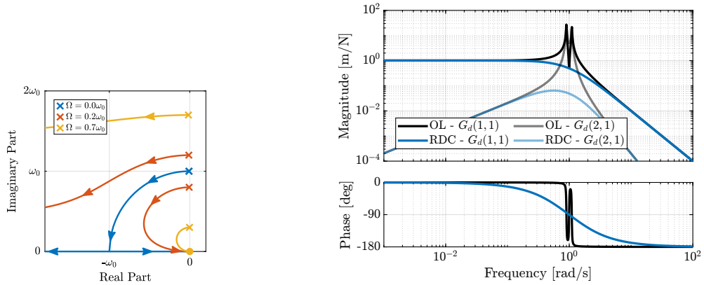
(a) Root locus for Relative Damping Control
