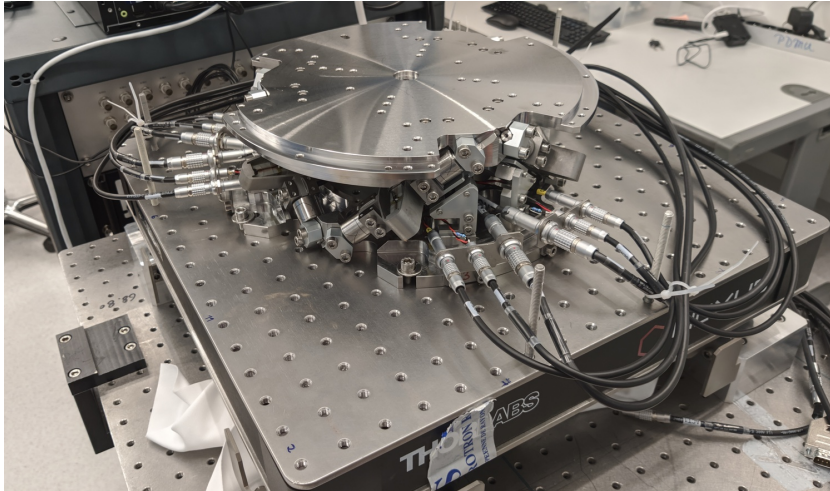
Figure 4.61: Mounted Nano-Hexapod on top of the suspended table.
