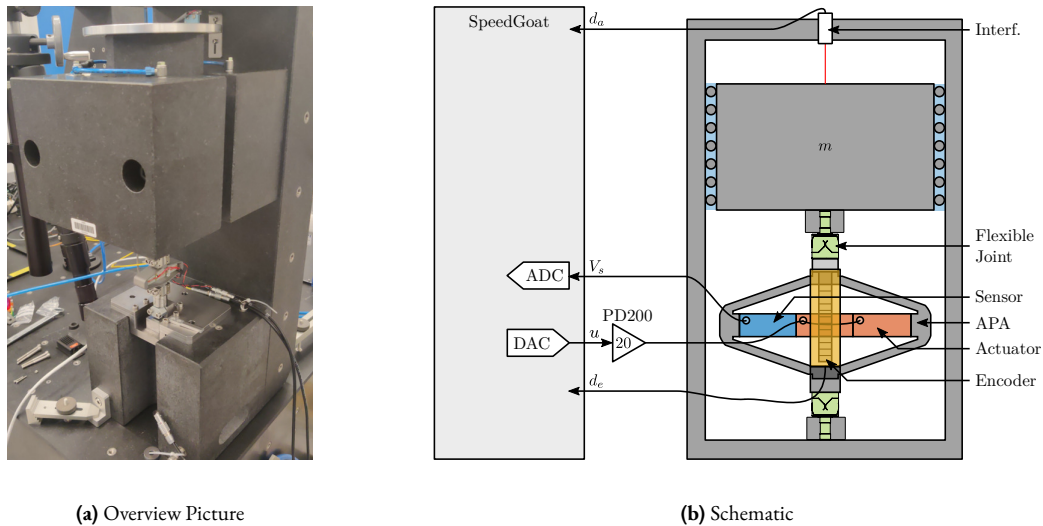
Figure 4.44: Experimental setup used to measure the dynamics of the struts.
