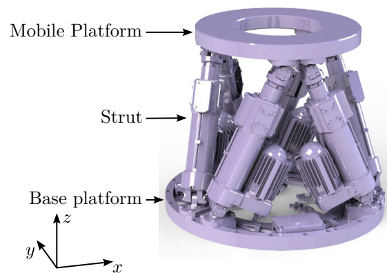
Figure 2.80: Positioning Hexapod.
