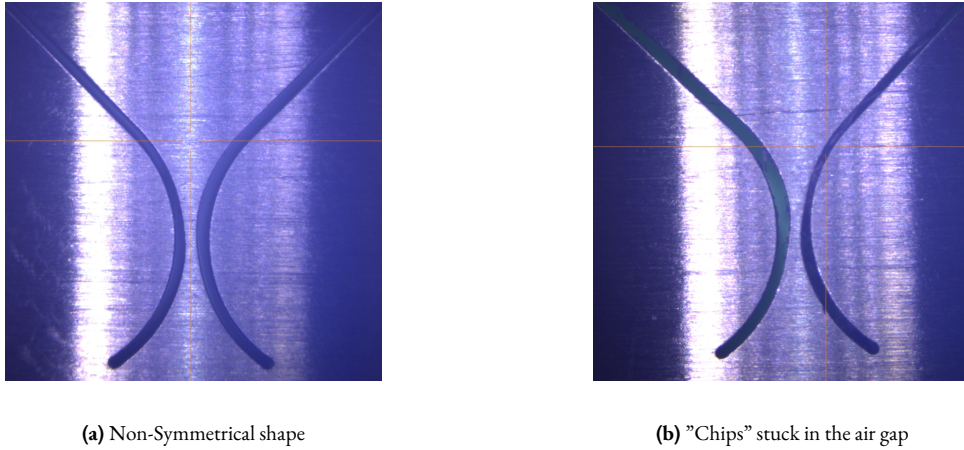
Figure 4.28: Example of two flexible joints that were considered unsatisfactory after visual inspection.
