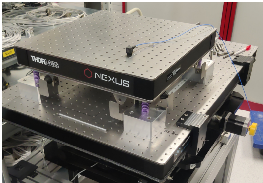
Figure 4.59: Mounted suspended table. Only 1 or the 15 accelerometers is mounted on top.
