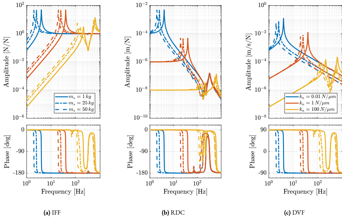
Figure 2.16: Plant dynamics for the three active damping techniques: IFF (a), RDC (b) and DVF (c). Three active platform stiffnesses ( k_n = 0.01 N/ \mu m in blue, k_n = 1 N/ \mu m in red and k_n = 100 N/ \mu m in yellow) and three sample's masses ( m_s = 1 kg: solid curves, m_s = 25 kg: dot-dashed curves, and m_s = 50 kg: dashed curves) are considered in each case.
