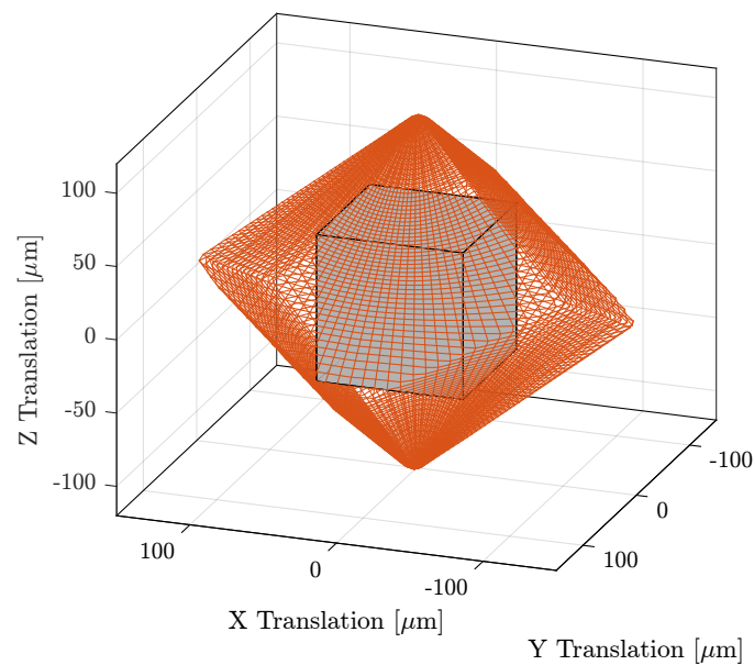
Figure 3.22: Specified translation mobility of the active platform (grey cube) and computed Mobility (red volume).
