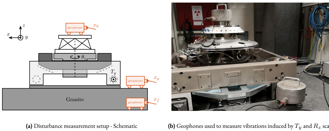
Figure 2.6: Identification of the disturbances coming from the micro-station. The measurement schematic is shown in (a). A picture of the setup is shown in (b).
