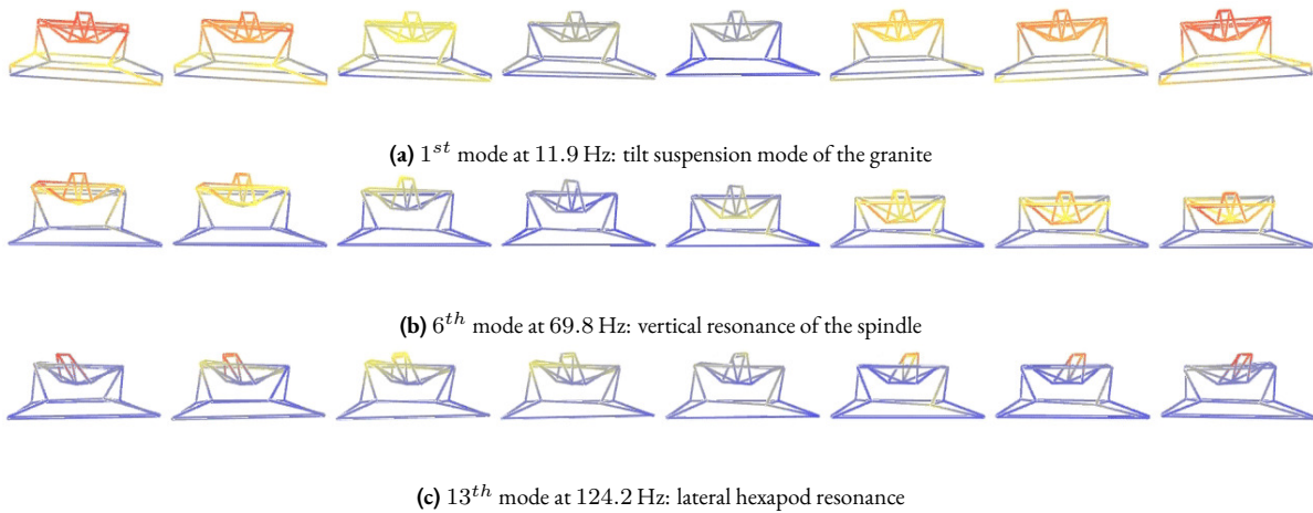
Figure 2.73: Three obtained mode shape animations.
