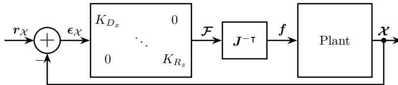
(b) Control in the Cartesian frame. J^{-T} is used to project forces and torques on each strut
