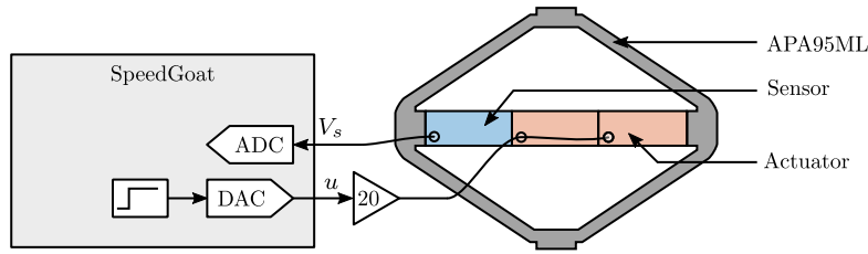
Figure 3.79: Schematic of the setup to validate the use of the ADC for reading the force sensor voltage.
