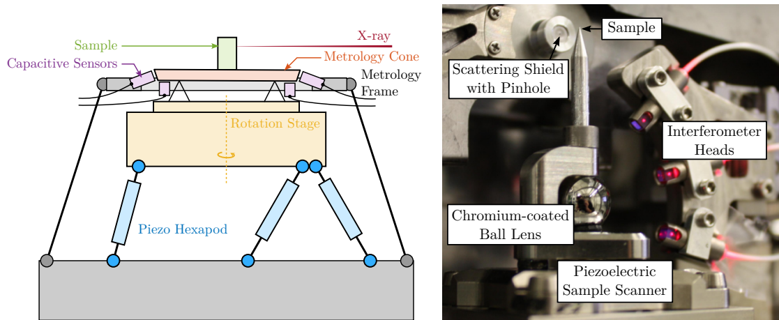
(a) Simplified schematic of ID16a end-station [148]
