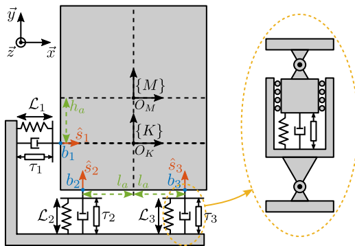
Figure 3.54: Model used to compare decoupling strategies.
