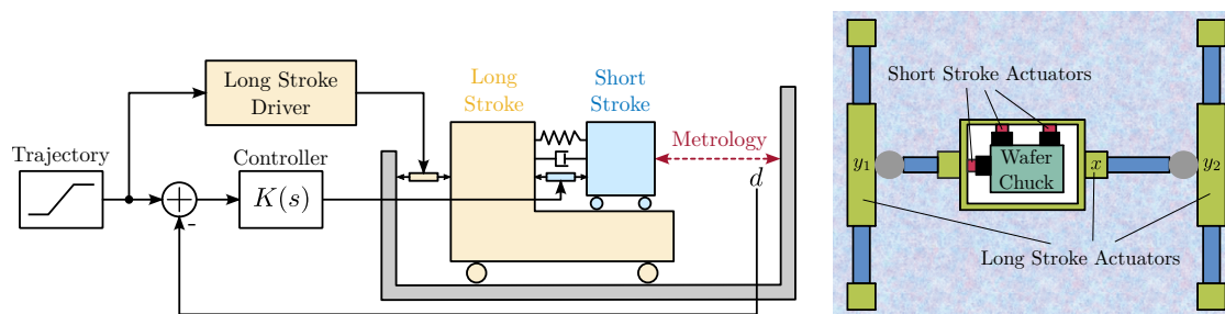
Figure 1.15: Schematic of a typical Long stroke-Short stroke control architecture (a). A 3-DoFs long stroke-short stroke is shown in (b) where y_1 , y_2 and x are 3-phase linear motors and short stroke actuators are voice coils.
