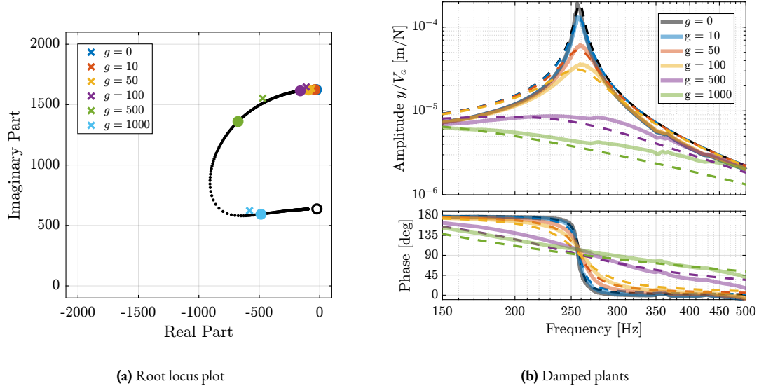
Figure 3.28: Results using Integral Force Feedback with the APA95ML. Closed-loop poles as a function of the controller gain g are predicted by the root locus plot (a). Circles are predictions from the model while crosses are poles estimated from the experimental data. Damped plants estimated from the model (dashed curves) and measured ones (solid curves) are compared in (b) for all tested controller gains.
