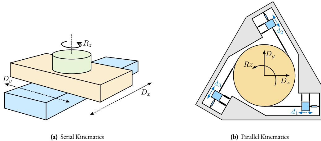
Figure 1.11: Two positioning platforms with D_x/D_y/R_z degrees of freedom. One is using serial kinematics (a), while the other uses parallel kinematics (b).
