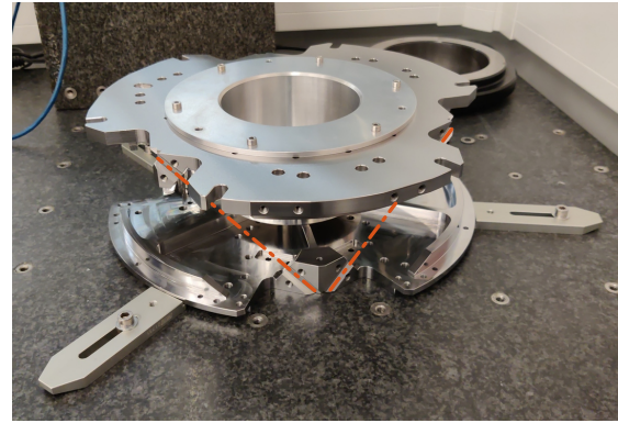
(b) Wanted coaxiality between strut interfaces
