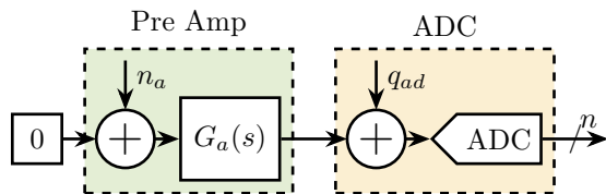
Figure 3.82: Measurement of the instrumentation amplifier input voltage noise.
