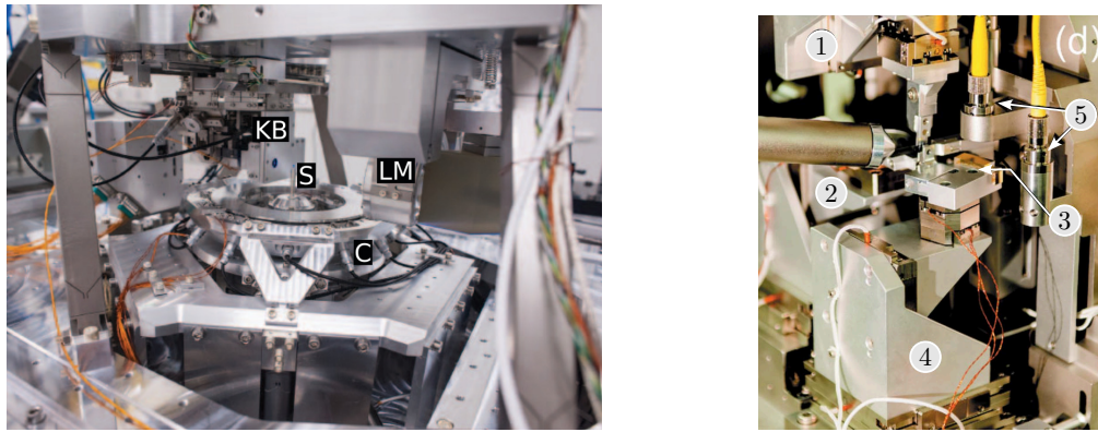
(a) ESRF ID16a - HPZ. KB is the focusing optics, S the sample, C the capacitive sensors and LM is the light microscope [148] (b) NSLS-II HXN - Microscope. 1 and 2 are focusing optics, 3 is the sample location, 4 the sample stage and 5 the interferometers [103]
