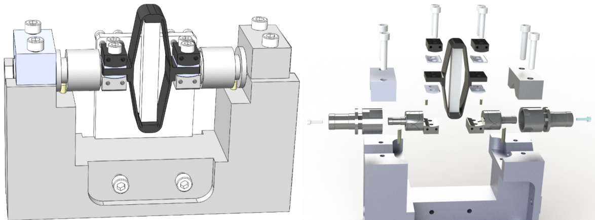
(a) 3D view of the mounting bench
