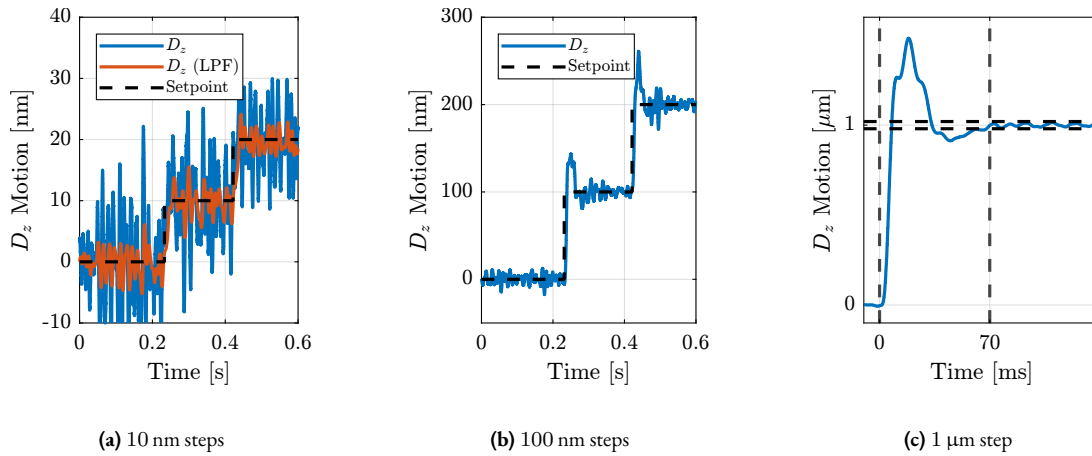
Figure 4.106: Vertical steps performed with the nano-hexapod. 10 nm steps are shown in (a) with the low-pass filtered data corresponding to an integration time of 50 ms. 100 nm steps are shown in (b). The response time to reach a peak-to-peak error of \pm 20 nm is \approx 70 ms as shown in (c) for a 1 \mu\text{m} step.
