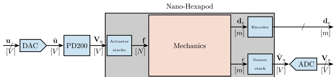
Figure 4.62: Block diagram of the studied system. The command signal is \mathbf{u} , and the measured signals are \mathbf{d}_e and \mathbf{V}_s .
