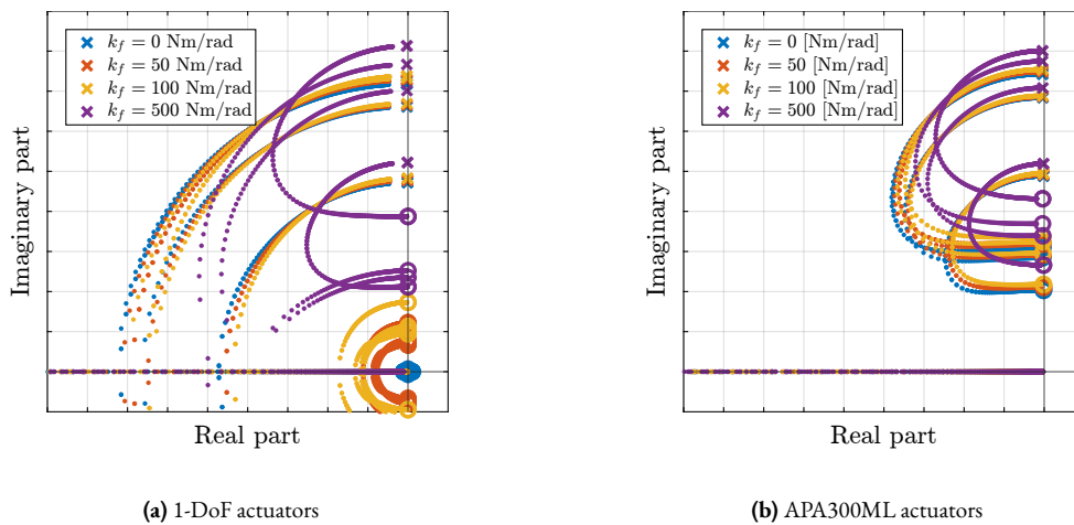
Figure 3.37: Effect of bending stiffness of the flexible joints on the attainable damping with decentralized IFF. For 1-DoF actuators (a), and with the 2-DoFs model of the APA300ML (b).
