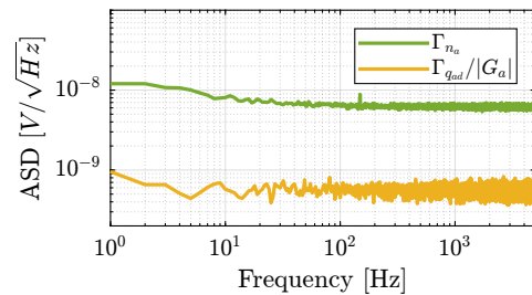
Figure 3.83: Obtained ASD of the instrumentation amplifier input voltage noise.
