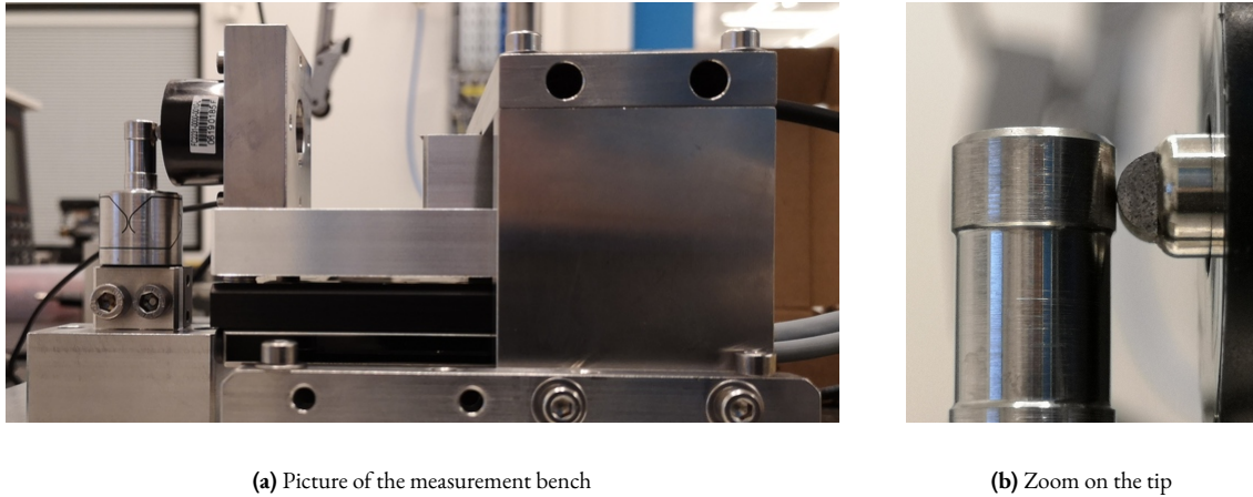
Figure 4.31: Manufactured test bench for compliance measurement of the flexible joints.
