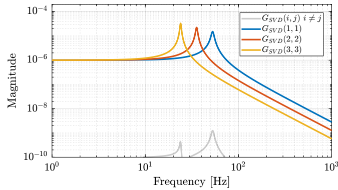
Figure 3.62: Plant dynamics G_{SVD}(s) obtained after decoupling using Singular Value Decomposition.
