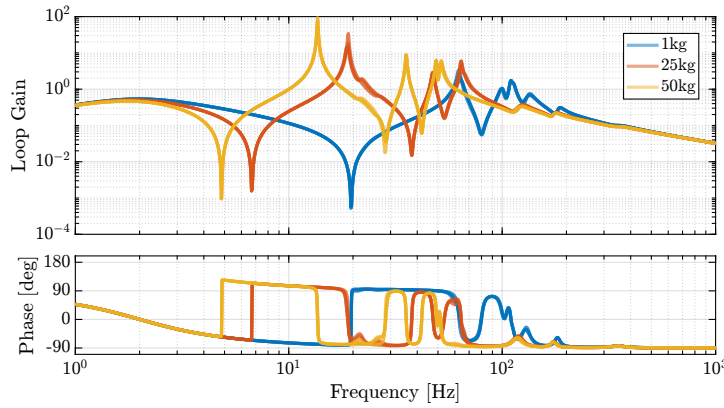
Figure 2.127: Loop gain for the decentralized IFF: K_{\text{IFF}}(s) \cdot \frac{f_{mi}}{f_i}(s) .
