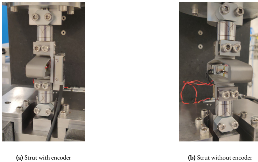
Figure 4.45: Strut fixed to the test bench with clamped flexible joints. The encoder can be fixed to the struts (a) or removed (b).
