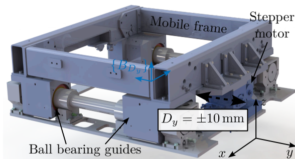
Figure 2.77: Translation Stage.
