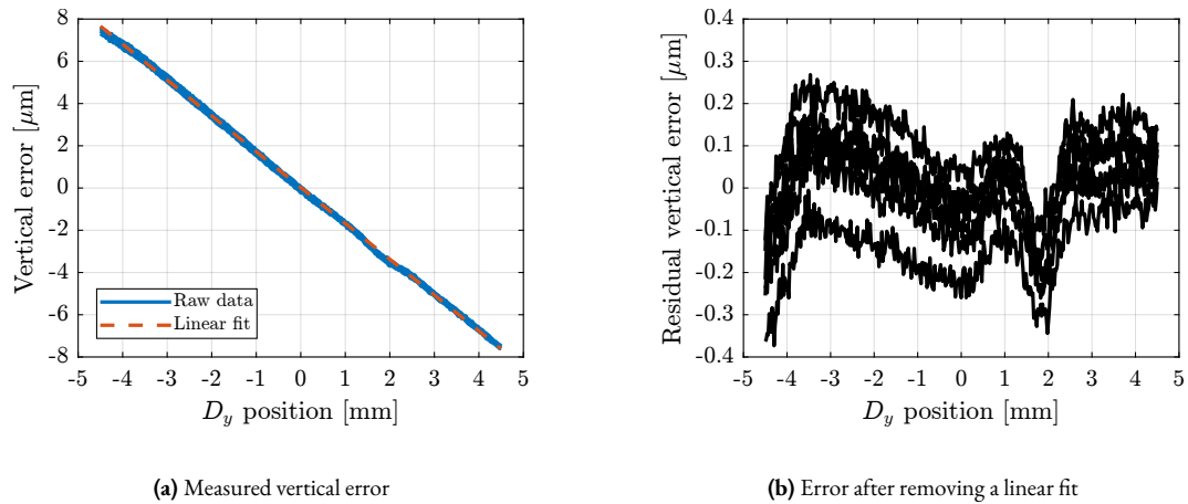
Figure 2.92: Measurement of the straightness (vertical error) of the translation stage (a). A linear fit is then removed from the data (b).
