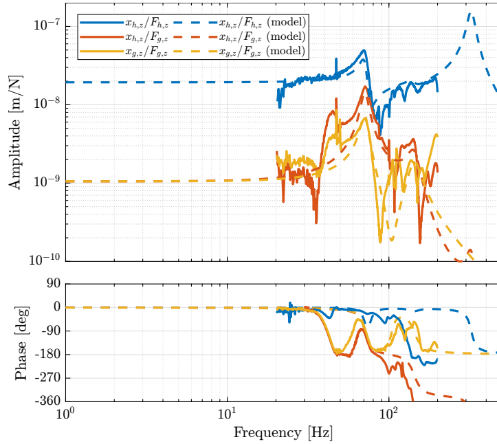
Figure 2.3: Comparison of the measured FRF and the uniaxial model dynamics.
