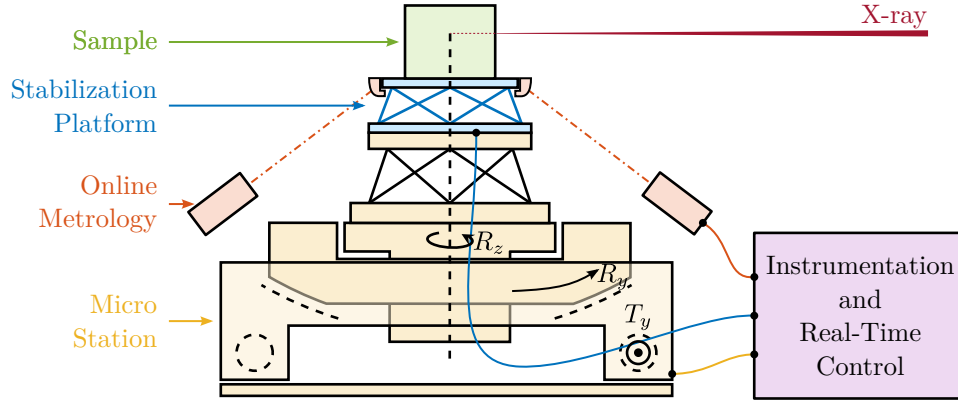
Figure 2.123: Schematic of the Nano Active Stabilization System.
