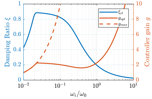
(b) Attainable damping ratio as a function of \omega_i/\omega_0 . Maximum and optical control gains are also shown
