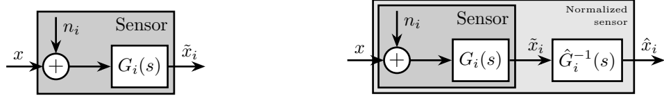
(a) Model with noise n_i and LTI transfer function G_i(s)
