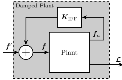
Figure 2.117: Schematic of the implemented decentralized IFF controller. The damped plant has input f' .
