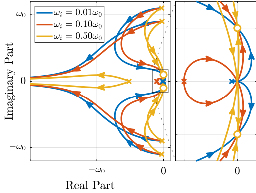
(a) Root locus
