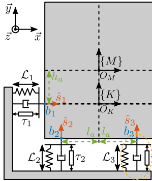
Figure 3.54: Model used to compare decoupling strategies.
