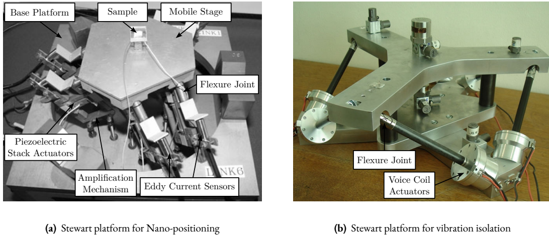
Figure 2.103: Two examples of Stewart platform. A Stewart platform based on piezoelectric stack actuators and used for nano-positioning is shown in (a) [47]. A Stewart platform based on voice coil actuators and used for vibration isolation is shown in (b) [108, 110]
