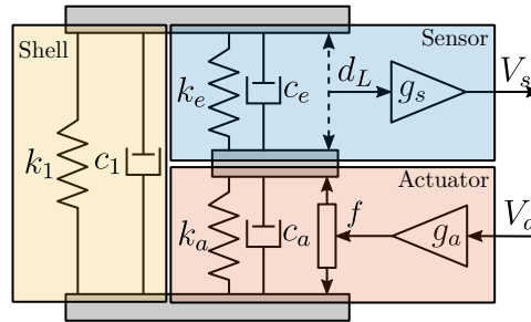
Figure 4.21: Schematic of the two degrees-of-freedom model of the APA300ML, adapted from [132]
