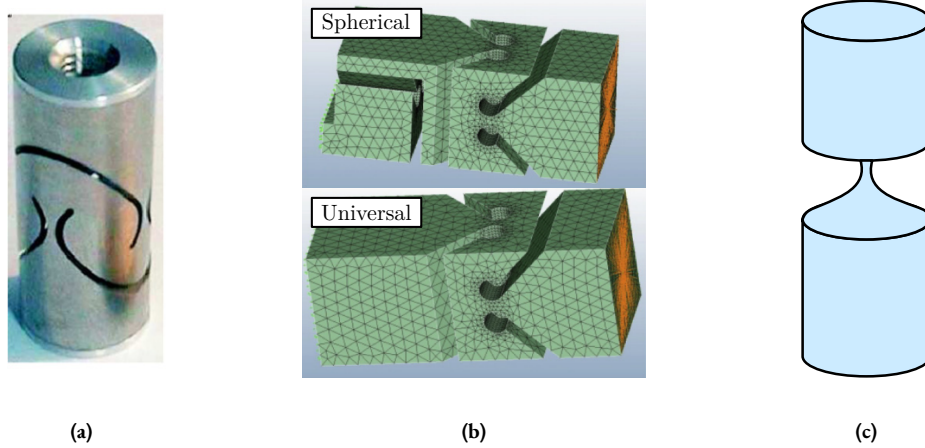
Figure 3.35: Example of different flexible joints geometry used for Stewart platforms. (a) Typical “universal” flexible joint used in [108]. (b) Torsional stiffness can be explicitly specified as done in [157]. (c) “Thin” flexible joints having “notch curves” are also used [37].
