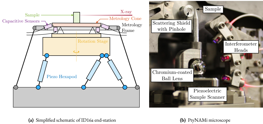
Figure 2.101: Example of two sample stages for tomography experiments. ID16a endstation [149] at the ESRF (a). PtyNAMi microscope [126, 127] at PETRA III (b)
