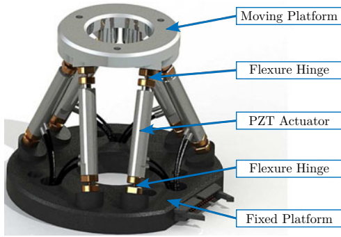
(a) Piezo based, for positioning purposes [37]
