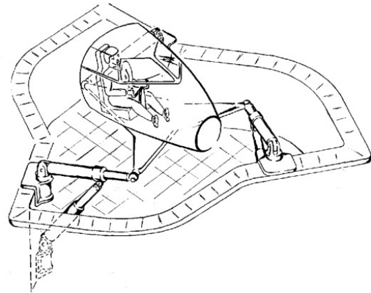
(b) Flight simulator proposed by Stewart [136]
