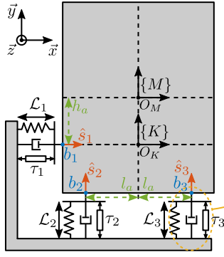
Figure 3.54: Model used to compare decoupling strategies
