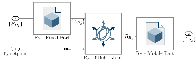
Figure 2.84: Example of a stage (here the tilt-stage) represented in the multi-body model software (SimScape). It is composed of two solid bodies connected by a 6-DoF joint. One joint DoF (here the tilt angle) can be imposed, the other DoFs are represented by springs and dampers. Additional disturbing forces for all DoF can be included
