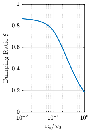
(a) Reduced damping ratio with increased cut-off frequency \omega_i
