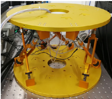
(c) Nanjing University - China [157]
