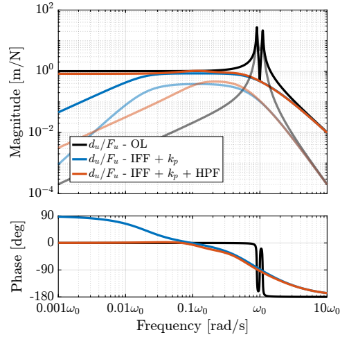
(b) Damped plant with the parallel stiffness, effect of the added HPF
