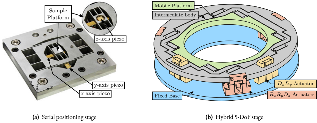
Figure 2.102: Examples of an XYZ serial positioning stage [76] (a) and of a 5-DoF hybrid (parallel/serial) positioning platform [130] (b).
