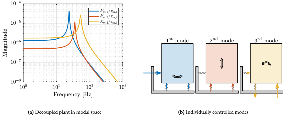
Figure 3.60: Plant using modal decoupling consists of second order plants (a) which can be used to individually address different modes illustrated in (b)
