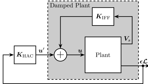
Figure 4.96: Block diagram of the implemented HAC-IFF controllers. The controller K_{\text{HAC}} is a diagonal controller with the same elements on every diagonal term K_{\text{HAC}} .
