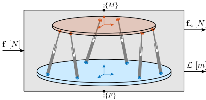
Figure 2.110: Nano-Hexapod plant with inputs and outputs. Frames \{F\} and \{M\} can be connected to other elements in the model.
