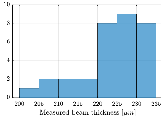
Figure 4.29: Histogram for the (16x2) measured beams' thicknesses
