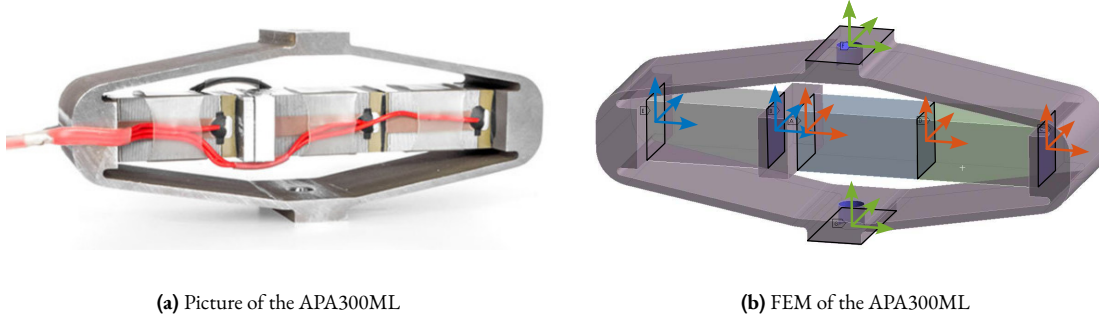
Figure 3.30: Amplified Piezoelectric Actuator APA300ML. Picture shown in (a). Frames (or “remote points”) used for the modal reduction are shown in (b).
