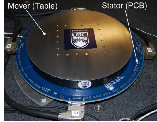
(b) Stage with infinite R_z rotation [38]
