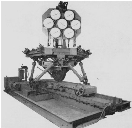
(a) Tyre test machine proposed by Gough [51]
