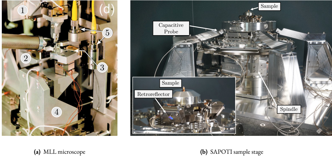
Figure 2.100: Example of sample stage with active XYZ corrections based on external metrology. The MLL microscope [101] at NSLS-II (a). Sample stage on SAPOTI beamline [50] at Sirius facility (b)
