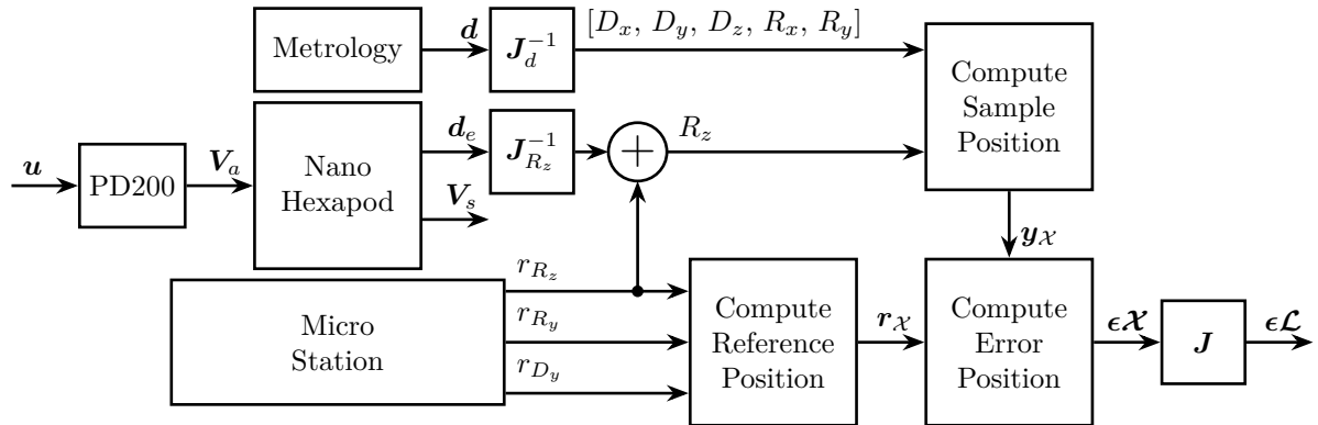
Figure 2.1: Schematic of the NASS plant
