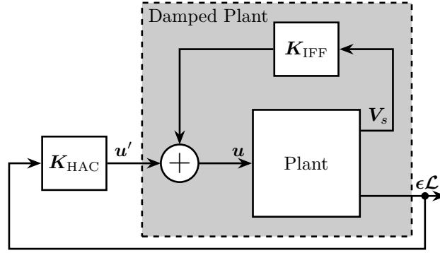
Figure 4.1: Block diagram of the implemented HAC-IFF controllers. The controller K_{HAC} is a diagonal controller with the same elements on every diagonal term K_{HAC} .
