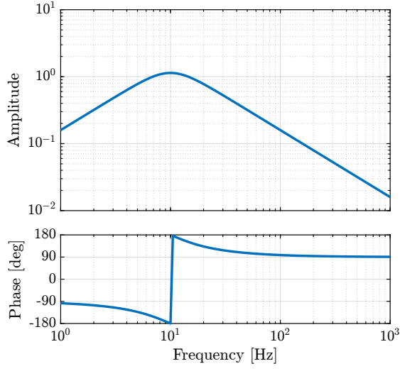
(a) Bode plot of K_{IFF}
