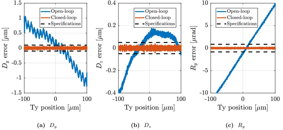
Figure 5.9: Open-Loop (in blue) and Closed-loop (i.e. using the NASS, in red) during a 10 \mu\text{m/s} scan with the T_y stage. Errors in D_y is shown in (a).
