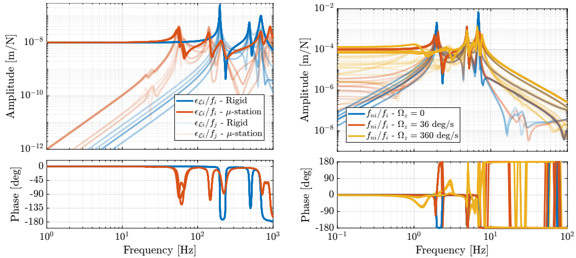
(a) k_a = 100 \text{ N}/\mu\text{m} - Coupling with the micro-station (b) k_a = 0.01 \text{ N}/\mu\text{m} - Effect of Spindle rotation
