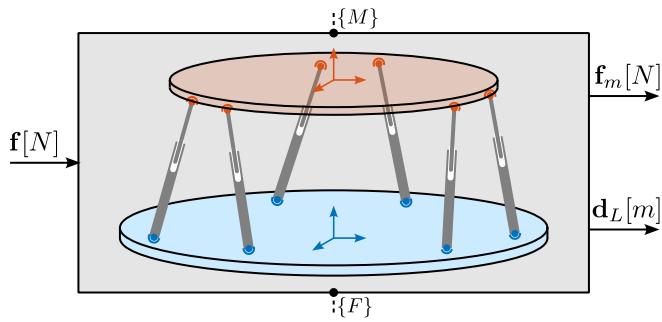
Figure 3.3: Nano-Hexapod plant with inputs and outputs. Frames \{F\} and \{M\} can be connected to other elements in the multi-body models.
