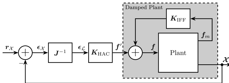
Figure 4.6: HAC-IFF control architecture with the High Authority Controller being implemented in the frame of the struts
