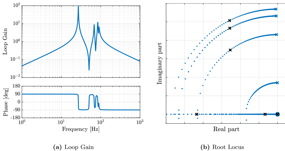
Figure 4.5: Decentralized IFF
