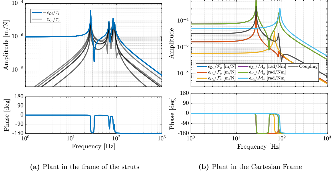
Figure 4.3: Bode plot of the transfer functions computed from the nano-hexapod multi-body model
