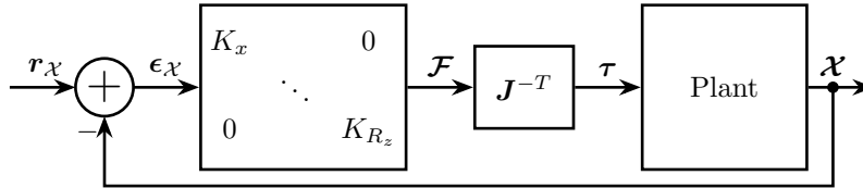
(b) Control in the Cartesian frame. J^{-T} is used to project force and torques on each strut
