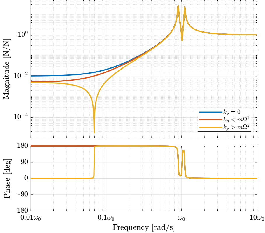
Figure 4.2: Effect of the parallel stiffness on the IFF plant: Bode plot of G_k(1,1) = f_u/F_u without parallel spring, with parallel spring stiffness k_p < m\Omega^2 and k_p > m\Omega^2 , \Omega = 0.1\omega_0
