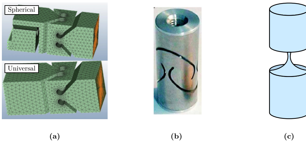
Figure 3.1: Example of different flexible joints geometry used for Stewart platforms. (a) [10]. (b) [11]. (c) [12].
