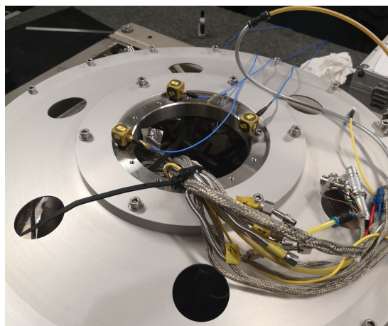
(b) Micro-Hexapod
