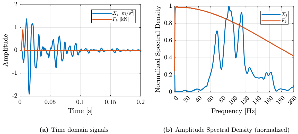
Figure 1.5: Raw measurement of the accelerometer (blue) and of the force sensor at the Hammer tip (red) (a). Computed Amplitude Spectral Densities of the two signals (normalized) (b)
