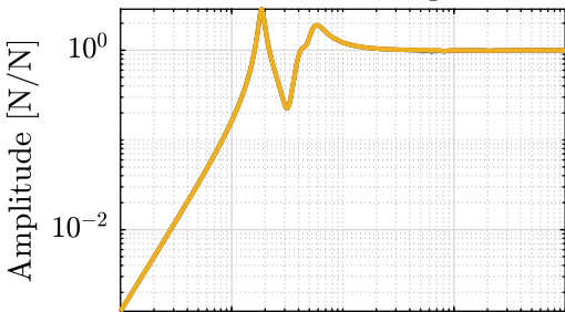
Soft Nano-Hexapod
