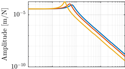
Soft Nano-Hexapod
