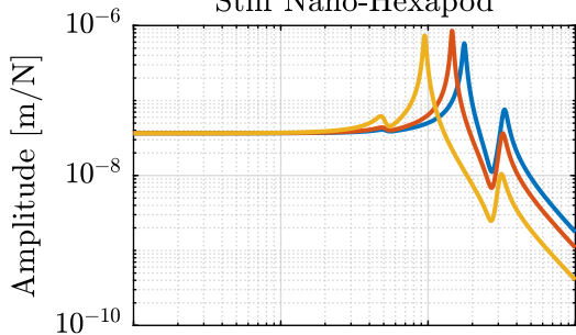
Stiff Nano-Hexapod
