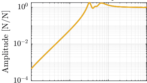
Soft Nano-Hexapod
