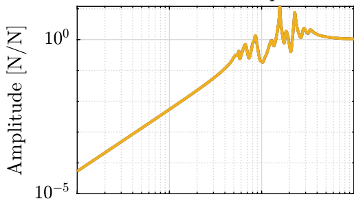
Stiff Nano-Hexapod
