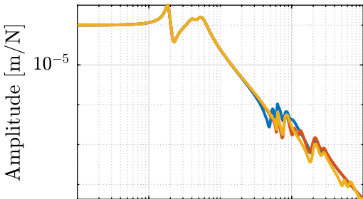
Soft Nano-Hexapod
