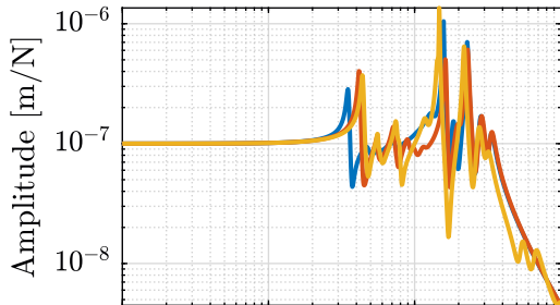
Stiff Nano-Hexapod
