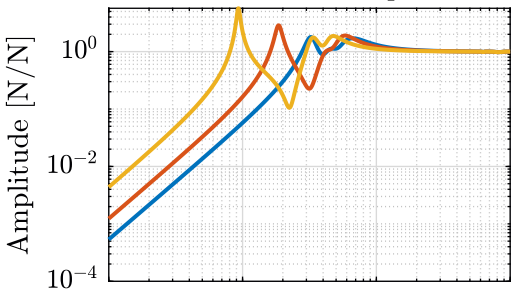
Soft Nano-Hexapod
