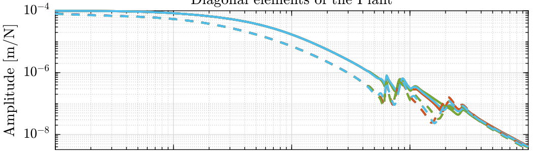
Diagonal elements of the Plant
