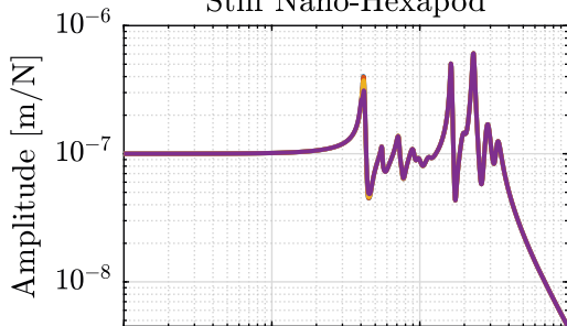
Stiff Nano-Hexapod
