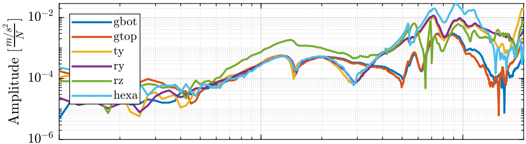
FRF between F_x and T_x
