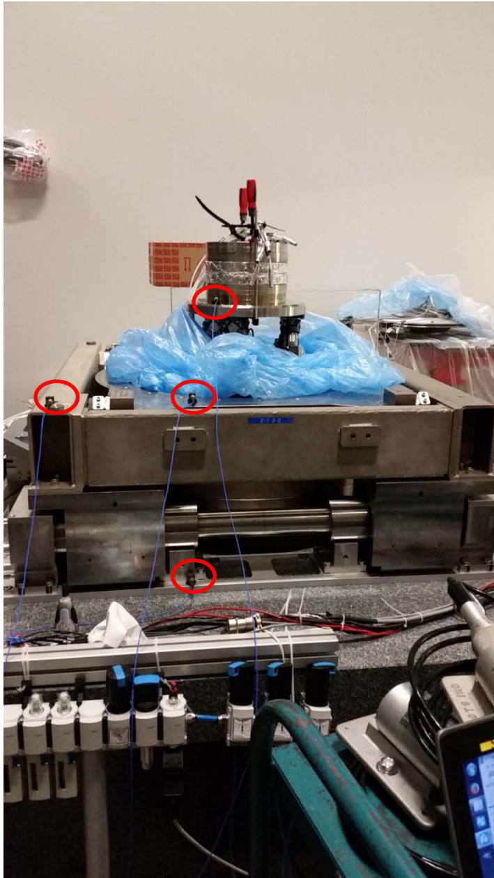
The 4 accelerometers
