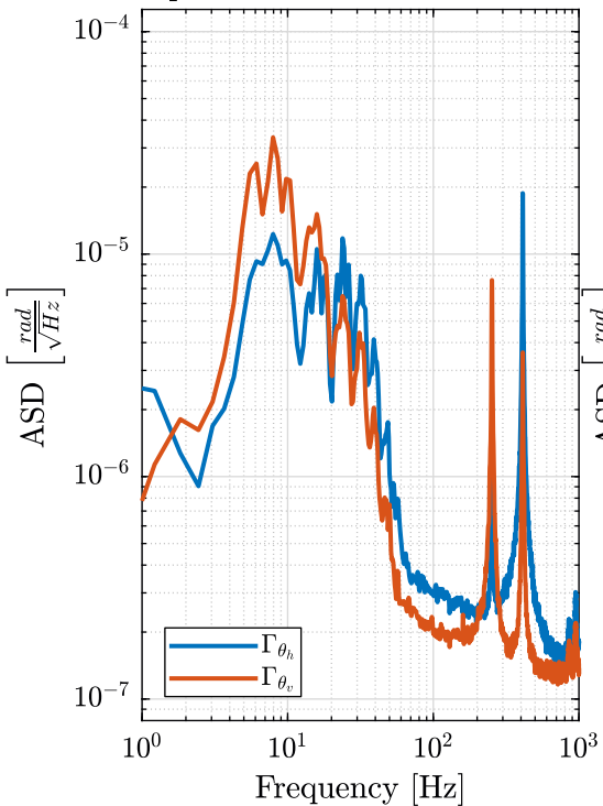
Newport Tilt - Horizontal Direction
