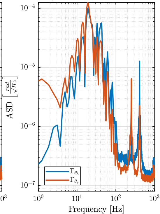
Newport Tilt - Vertical Direction
