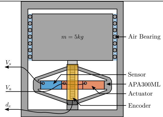
Figure 7: Schematic of the bench used to identify the APA dynamics
