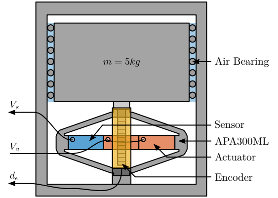
Figure 6: Schematic of the bench used to identify the APA dynamics.
