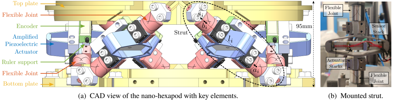
Figure 4: Nano-hexapod: A Stewart platform architecture.
