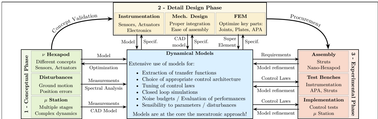
Figure 2: Overview of the mechatronics approach used for the design of the NASS.
