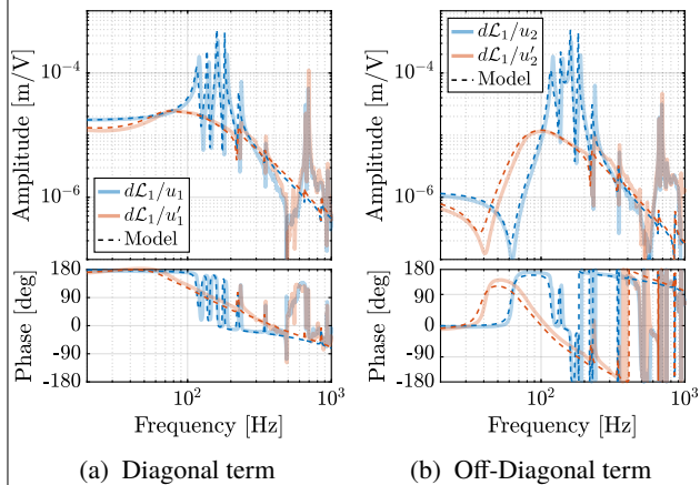
Figure 9: Transfer functions from actuator to encoder with and without the active damping technique applied.
