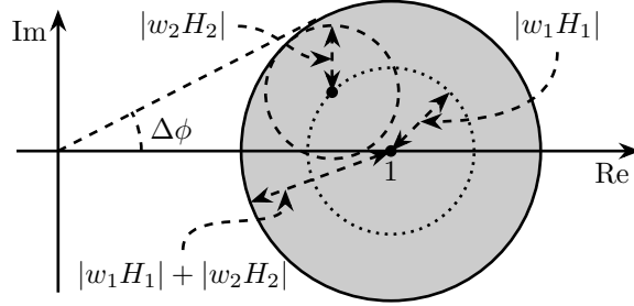
Figure 3: Uncertainty region of the super sensor dynamics in the complex plane (solid circle). The contribution of both sensors 1 and 2 to the uncertainty are represented respectively by a dotted and a dashed circle
