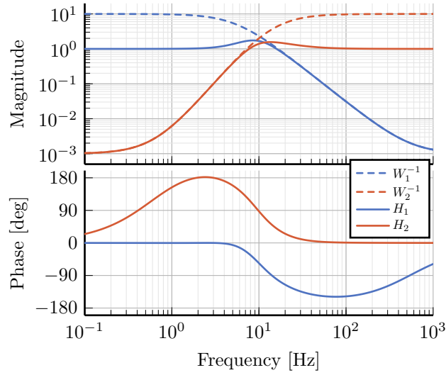
Figure 6: Frequency response of the weighting functions and complementary filters obtained using \mathcal{H}_\infty synthesis
