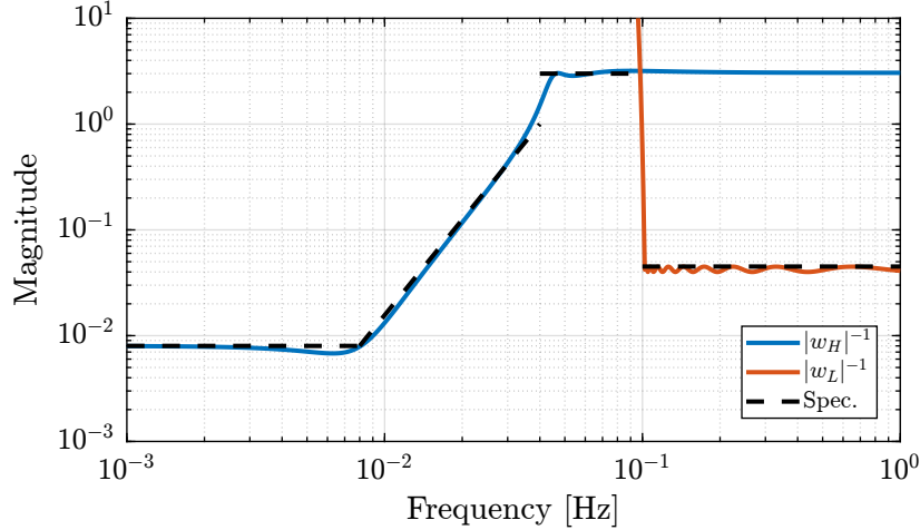
Figure 10: Specifications and weighting functions magnitudes
