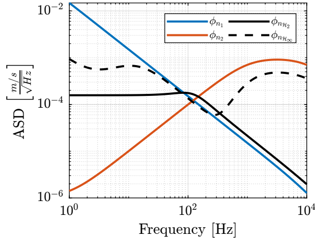
Figure 20 – Power Spectral Density of the estimated \hat{x} using the two sensors alone and using the \mathcal{H}_\infty synthesis
