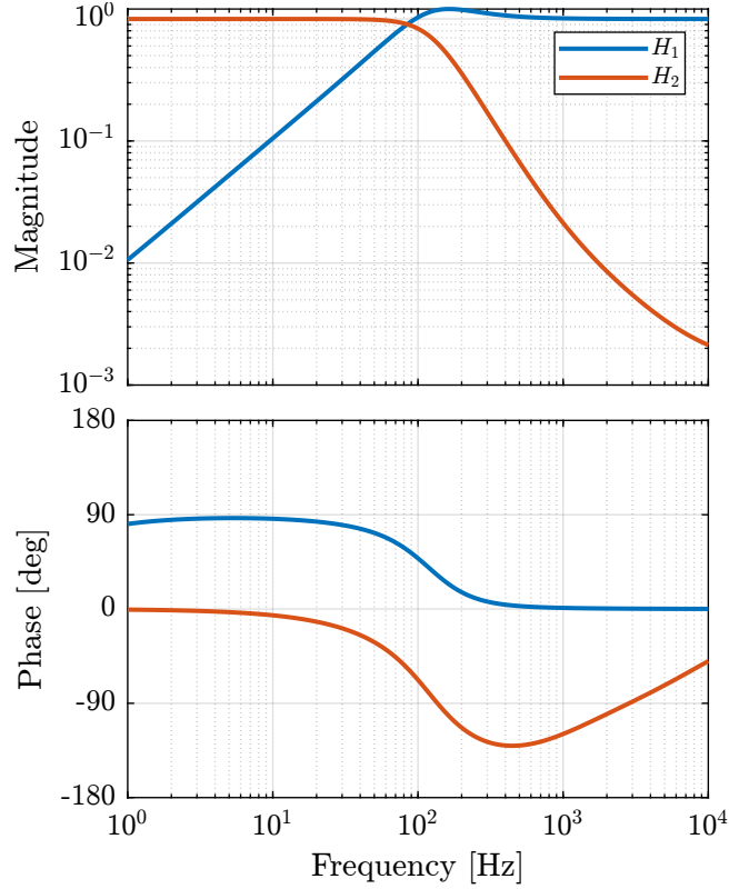
Figure 10 – Obtained complementary filters using the \mathcal{H}_2 Synthesis
