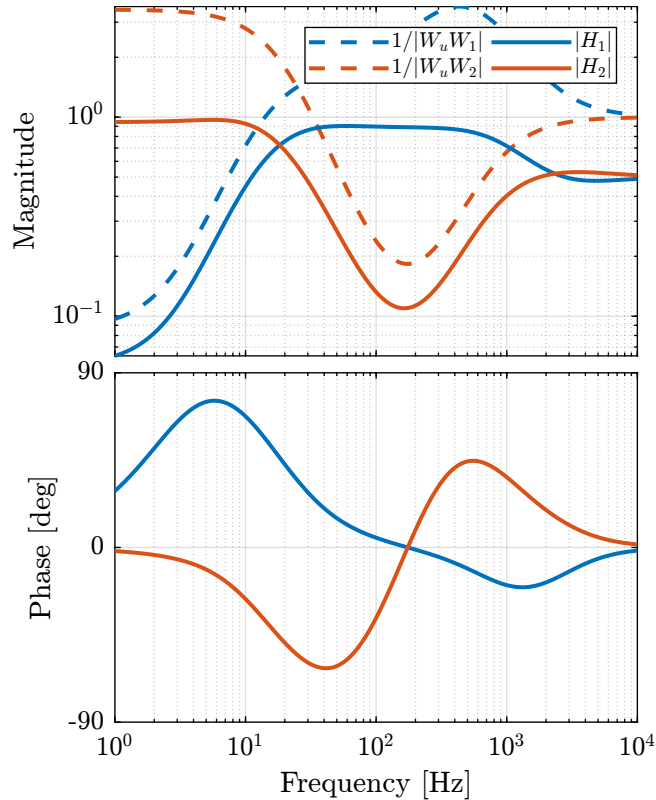
Figure 18 – Obtained complementary filters using the \mathcal{H}_\infty Synthesis
