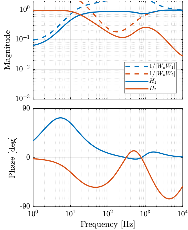
Figure 23 – Obtained complementary filters after mixed \mathcal{H}_2/\mathcal{H}_\infty synthesis
