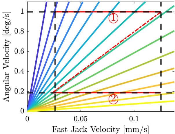
Constant Bragg Angular Velocity
