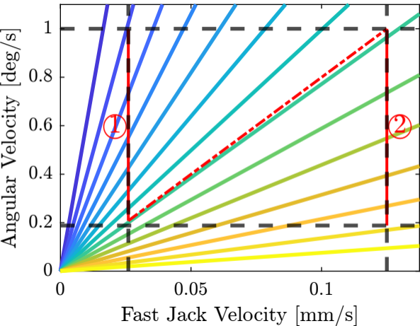
Constant Fast Jack Velocity
